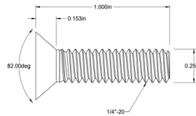
Divider Screws
