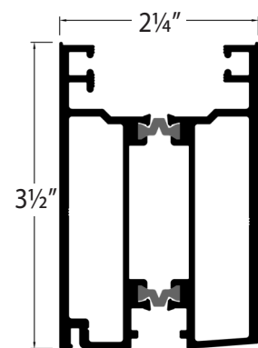
ACTIVE STILE E0025
