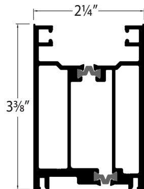
RECESSED STILE E0022
