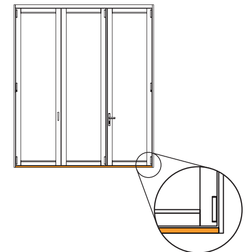
REDUCER BARS
