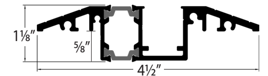
MODIFIED STANDARD SILL | E0110
