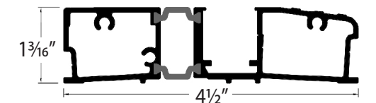
STANDARD SILL | E0023
