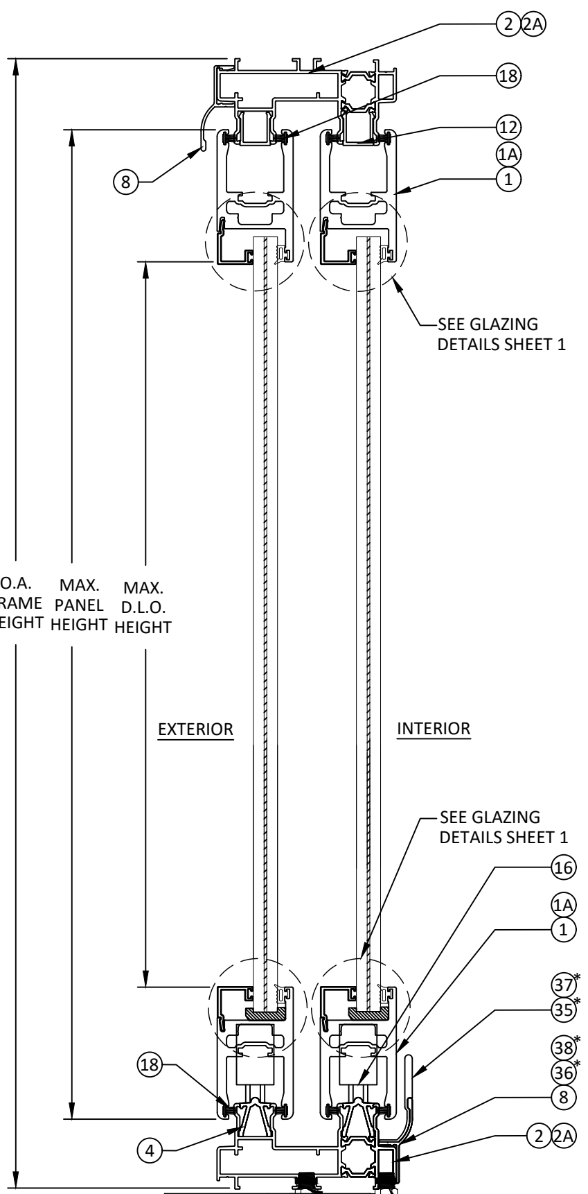
C 5 VERTICAL SECTION SLIDING GLASS DOOR OPTIONAL SUNKEN SILL 2 TRACKS SHOWN, 3 TRACKS QUALIFIED
