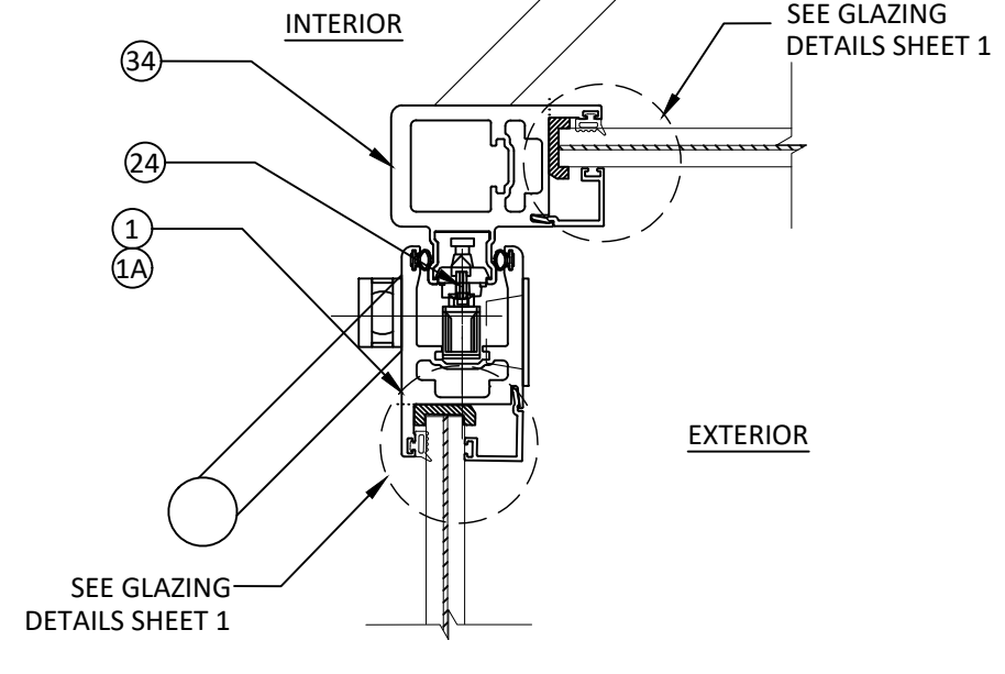
C 6 HORIZONTAL SECTION INSIDE CORNER DETAIL
