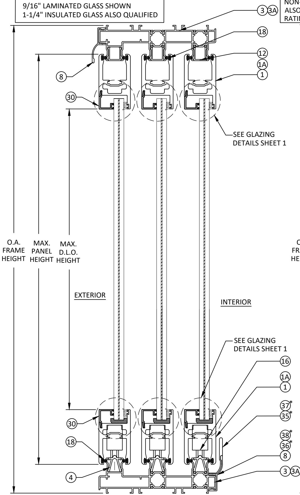
A 5 VERTICAL SECTION SLIDING GLASS DOOR 3 TRACKS
