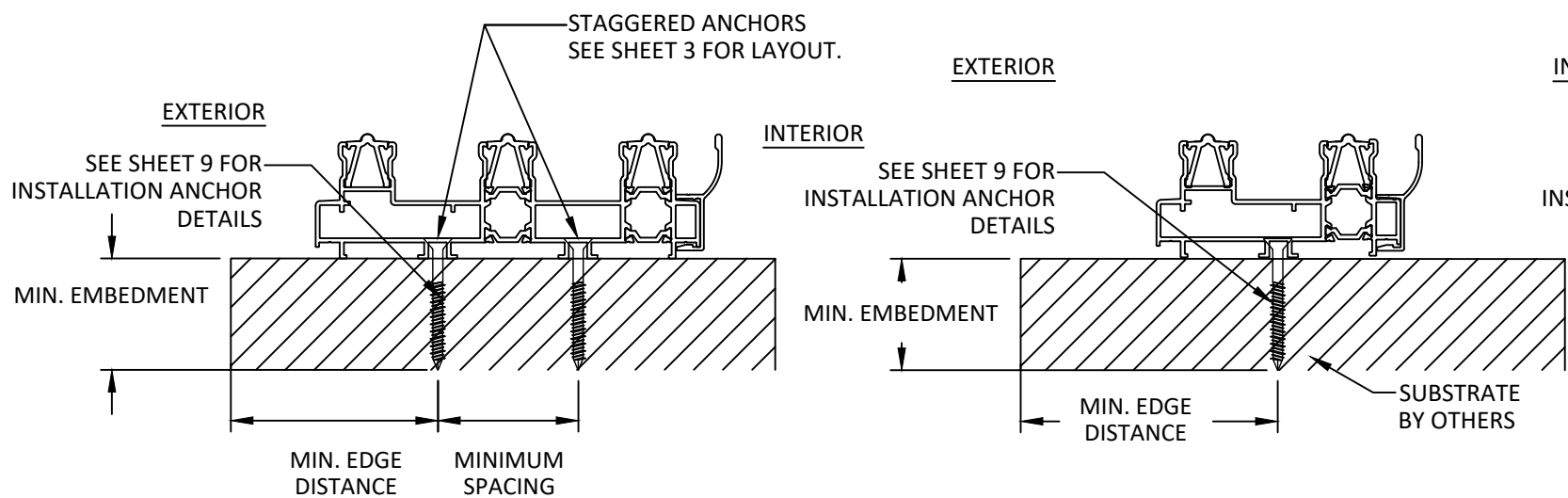
F 8 ANCHOR DETAIL THROUGH FRAME INSTALLATION (SILL) 2 TRACKS
