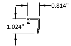
30 9/16" GLAZING BEAD 6063-T5
