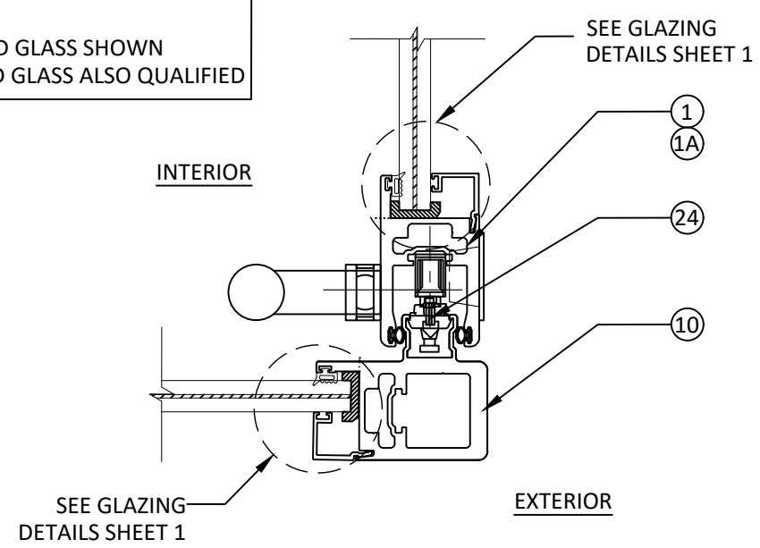
B 6 HORIZONTAL SECTION OUTSIDE CORNER DETAIL
