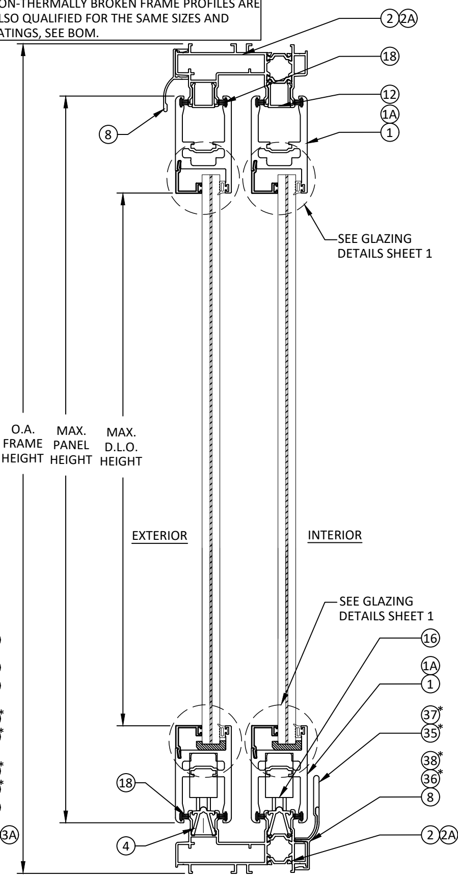
B 5 VERTICAL SECTION SLIDING GLASS DOOR 2 TRACK
