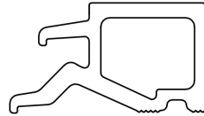
E0225-B 9/16" Reducer (9/16" Glass)
