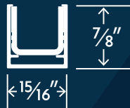
CHANNEL SILL Not Thermally Broken
