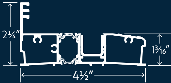
STANDARD SILL Water-Rated
