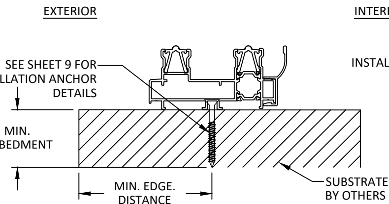
F 8 ANCHOR DETAIL THROUGH FRAME INSTALLATION (SILL) 2 TRACKS
