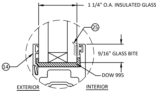
GLAZING DETAIL 2
