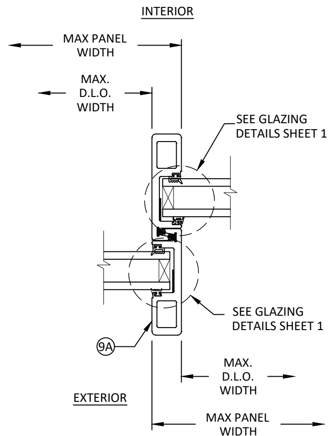
C HORIZONTAL SECTION 7 ALTERNATE INTERLOCK
