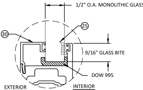
GLAZING DETAIL 1
