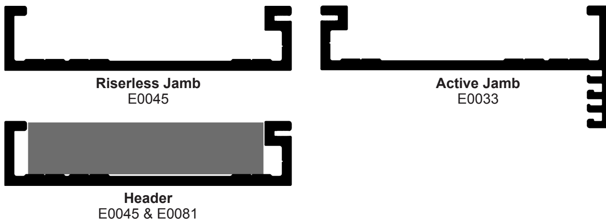
FIGURE B.1: JAMBS & HEADER
