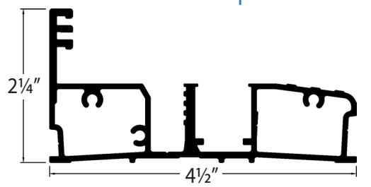
STANDARD SILL | E0037
