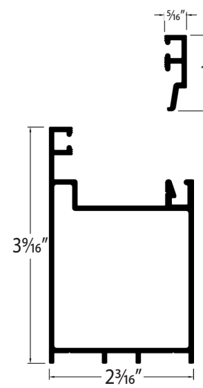
RAIL E0035
