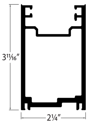
RECESSED STILE E0036
