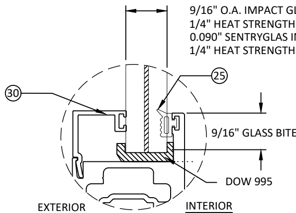
GLAZING DETAIL 1
