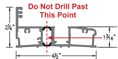
Standard Sill
