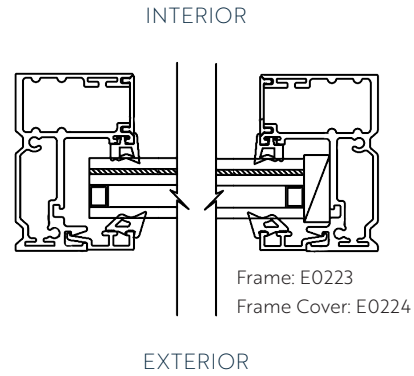
Top Down Cross Section
