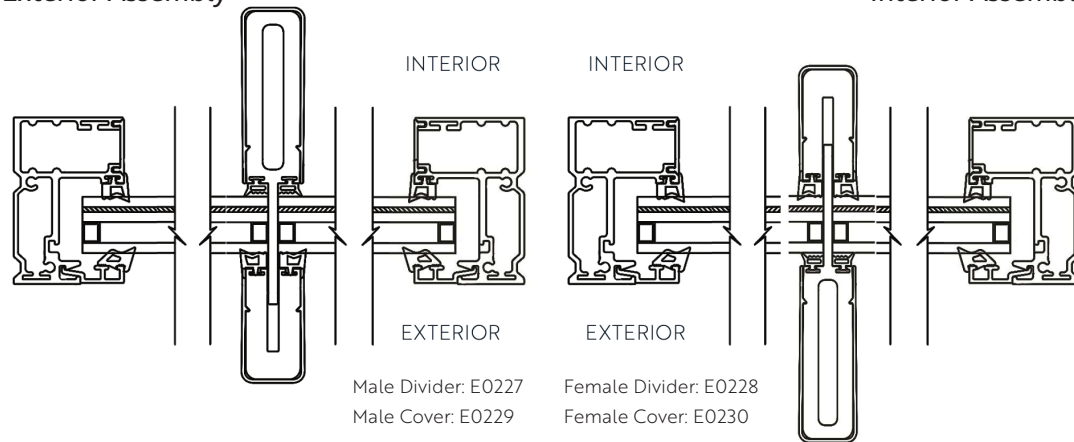
Exterior Assembly
