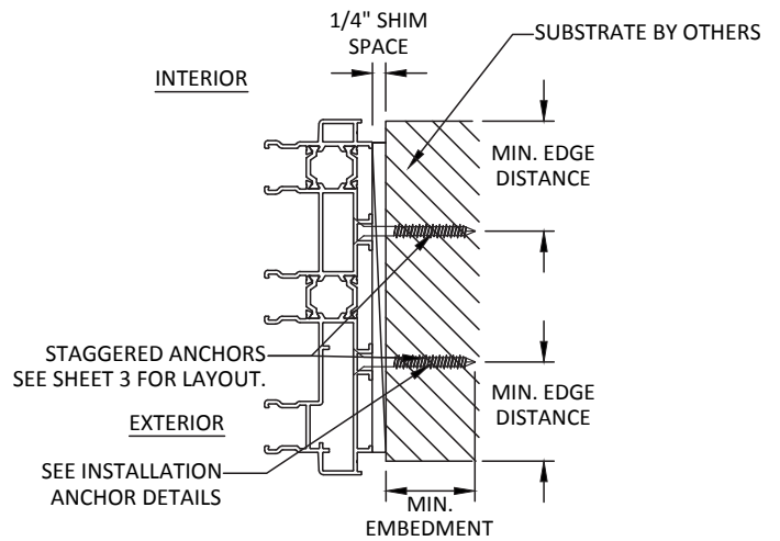
B 9 ANCHOR DETAIL THROUGH FRAME (JAMB) 3 TRACK
