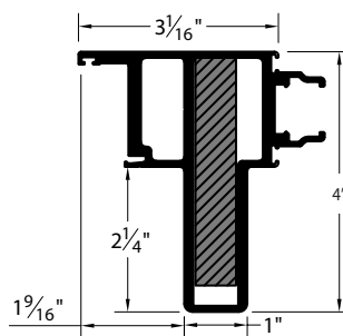
Center Meet Astragal E0094
