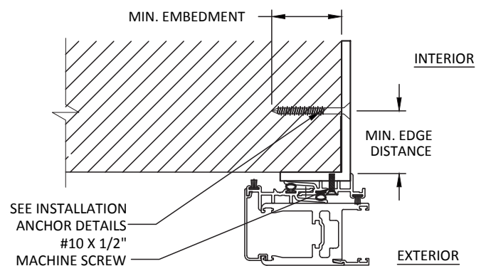
D 9 ANCHOR DETAIL OUTSIDE POCKET BRACKET INSTALLATION
