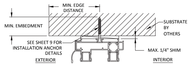
B 8 ANCHOR DETAIL THROUGH FRAME INSTALLATION (HEAD) 2 TRACKS
