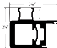
Outside Corner Astragal E0014
