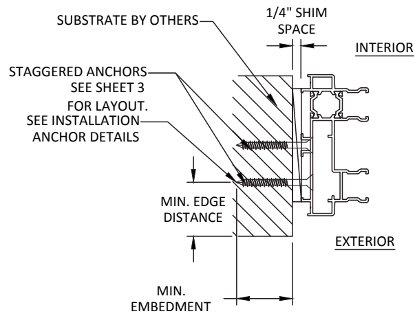
A 9 ANCHOR DETAIL THROUGH FRAME (JAMB) 2 TRACK
