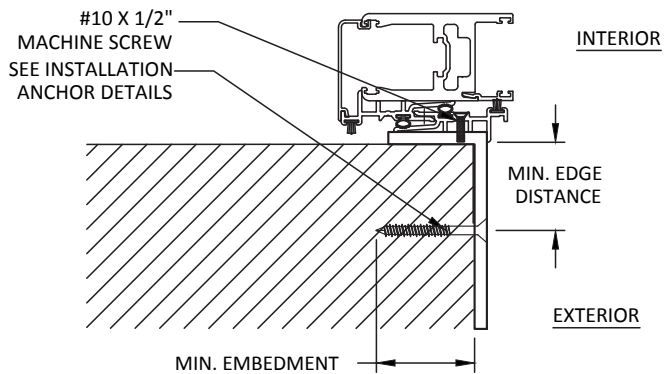
C 9 ANCHOR DETAIL INSIDE POCKET BRACKET INSTALLATION
