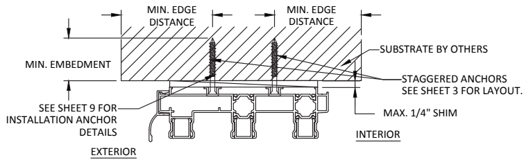
A 8 ANCHOR DETAIL THROUGH FRAME INSTALLATION (HEAD) 3 TRACKS
