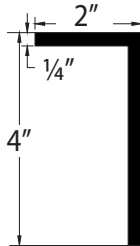
P HOOK MOUNT | E0096
