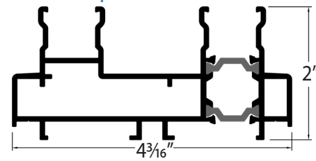
2 TRACK ADD ON | E0167
