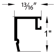
9/16" BEAD COMBO | E0093
