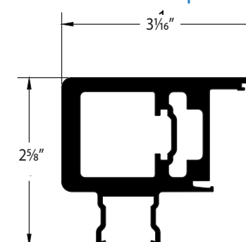
INSIDE CORNER ASTRAGAL | E0124
