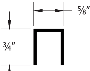
TRACK FILLER | E0109
