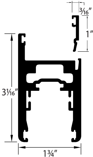
SASH | E0008 GLAZING BEAD | E0064
