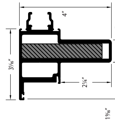
OUTSIDE CORNER ASTRAGAL | E0014
