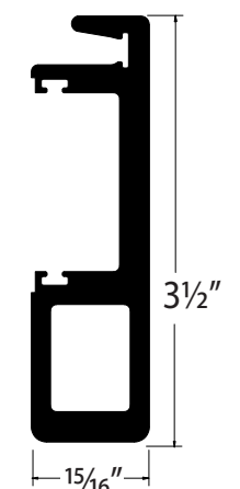
SLIM-LOCK INTERLOCK (OPTIONAL, NON-IMPACT) | E0240
