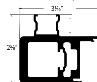
OUTSIDE CORNER ASTRAGAL | E0014
