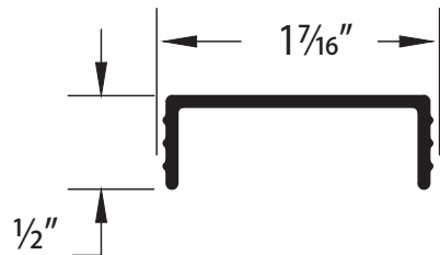
TRACK FILLER | E0109
