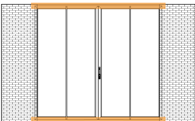
CONDENSATION DRAINS
