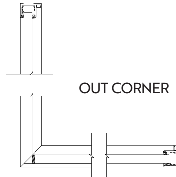
Top Down Cross Section
