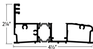
Standard Sill E0023
