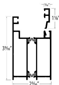
Rail & Snap Bead Rail: E0024 Bead: E0010
