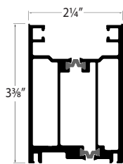
Recessed Stile E0022
