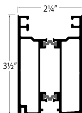
Active Stile E0025
